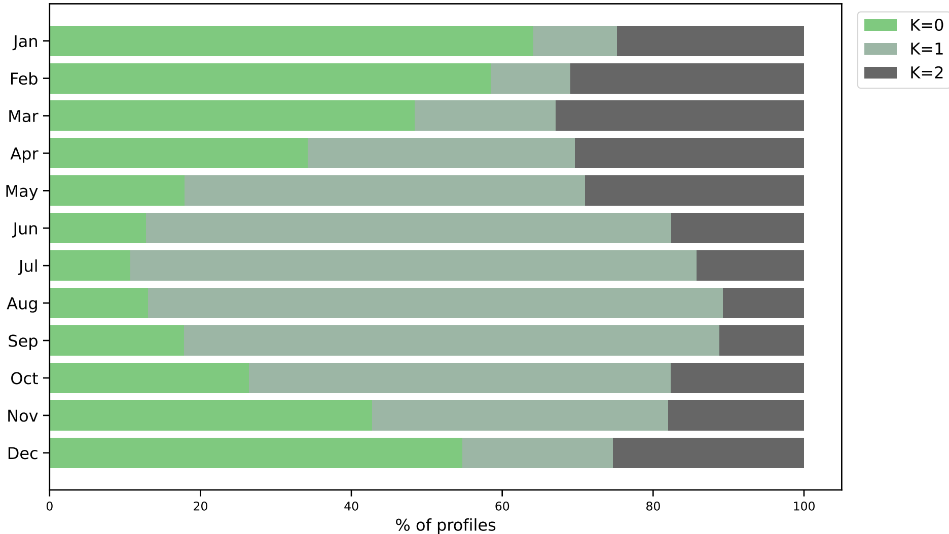
Percentage of profiles in each class by month for: 3900070
