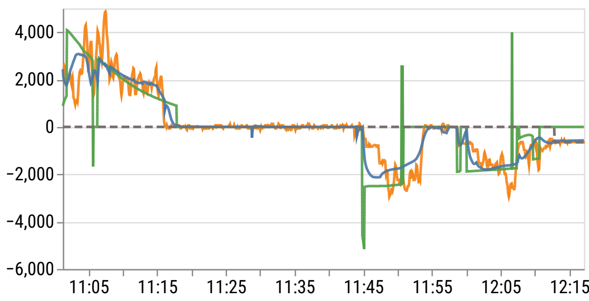
vertical speed (in ft/min)
