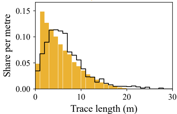
ADFNE, median 4.6 m
