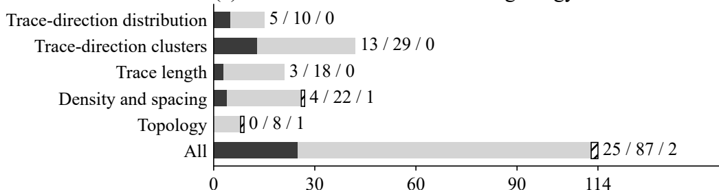
(a) Full EVAE vs EVAE without geology-informed terms
