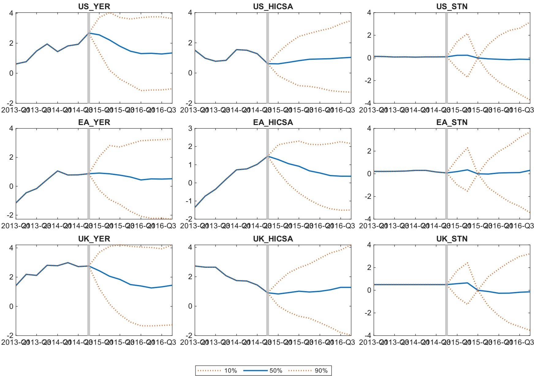
Conditional forecast (percentiles) [1]
