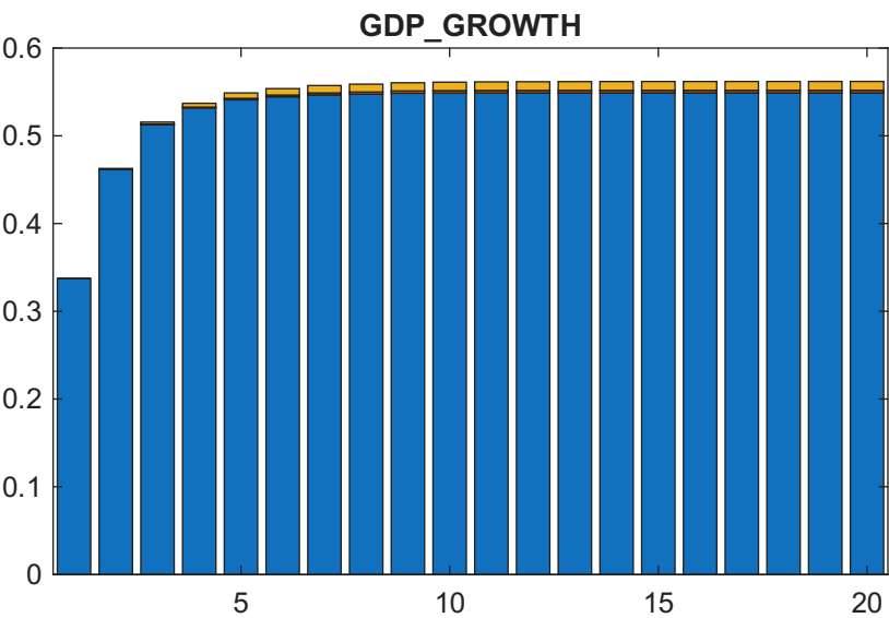
Forecast error variance decomposition (median) [1]
