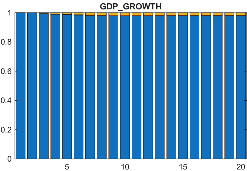
Forecast error variance decomposition (relative, median) [1]
