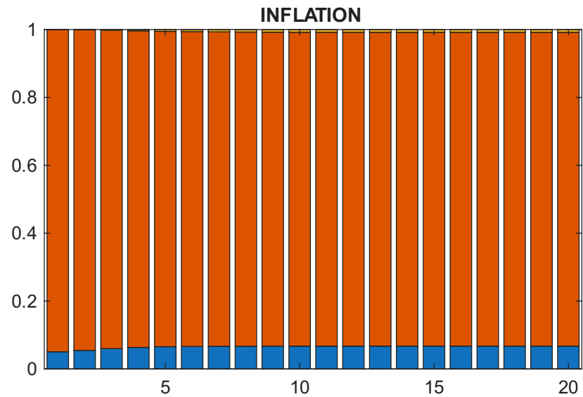
Forecast error variance decomposition (relative, median) [1]
