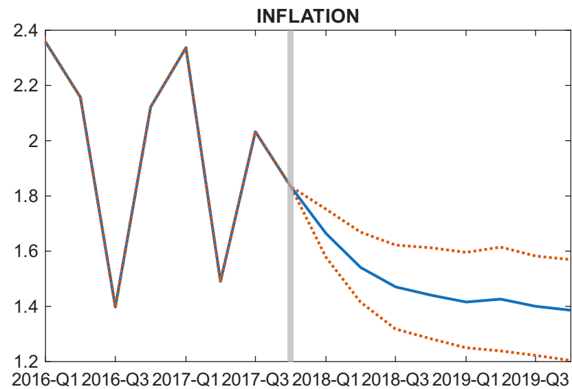
Conditional forecast (percentiles) [1]
