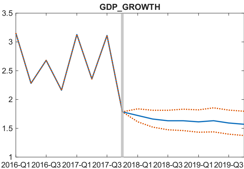
Conditional forecast (percentiles) [1]
