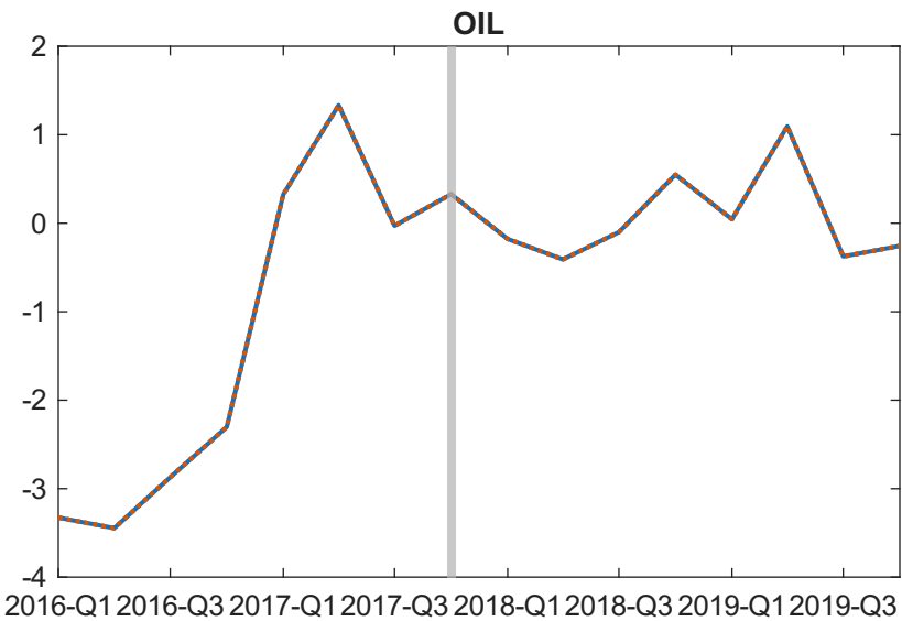
Structural model forecast (percentiles) [3]
