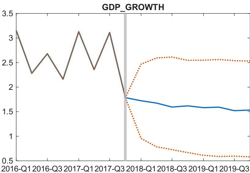
Structural model forecast (percentiles) [1]
