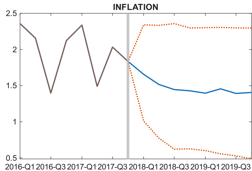
Structural model forecast (percentiles) [1]
