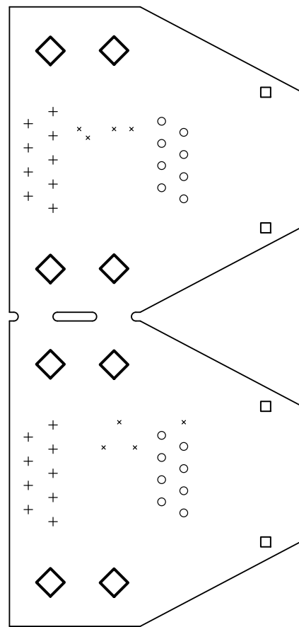
Drill Map:
