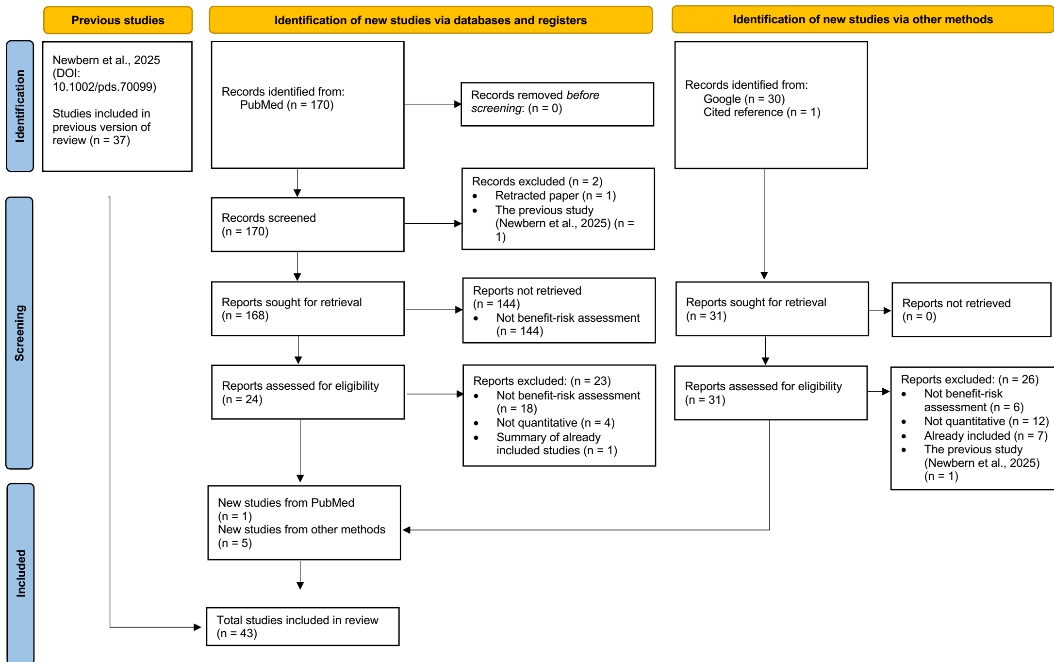
Figure S1. PRISMA flowchart
