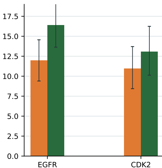
EF1%
