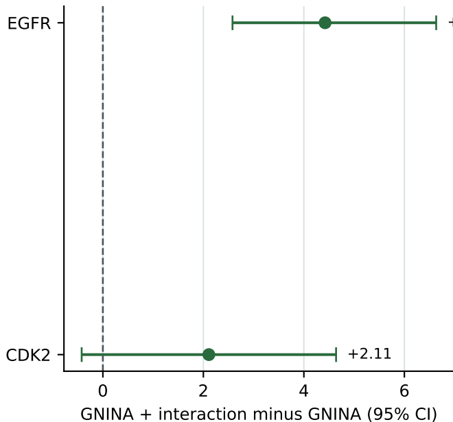
EF1% difference
