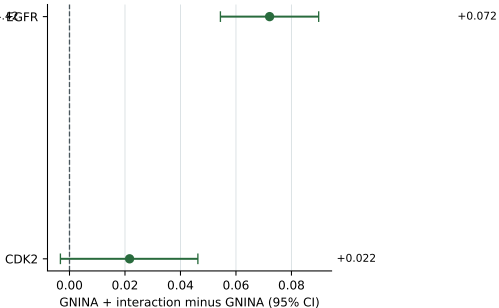
BEDROC difference
