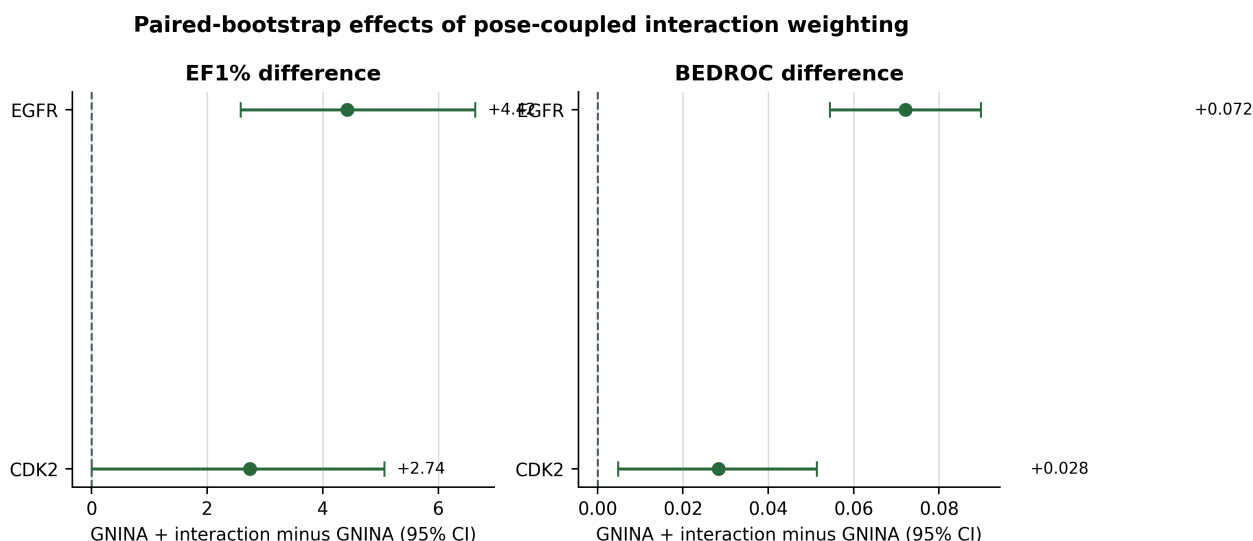
Figure 2: Paired-bootstrap effects of pose-coupled interaction weighting for EGFR and CDK2. Points show coupled-minus-GNINA estimates and horizontal bars show paired 95% confidence intervals; the dashed line denotes no difference.
