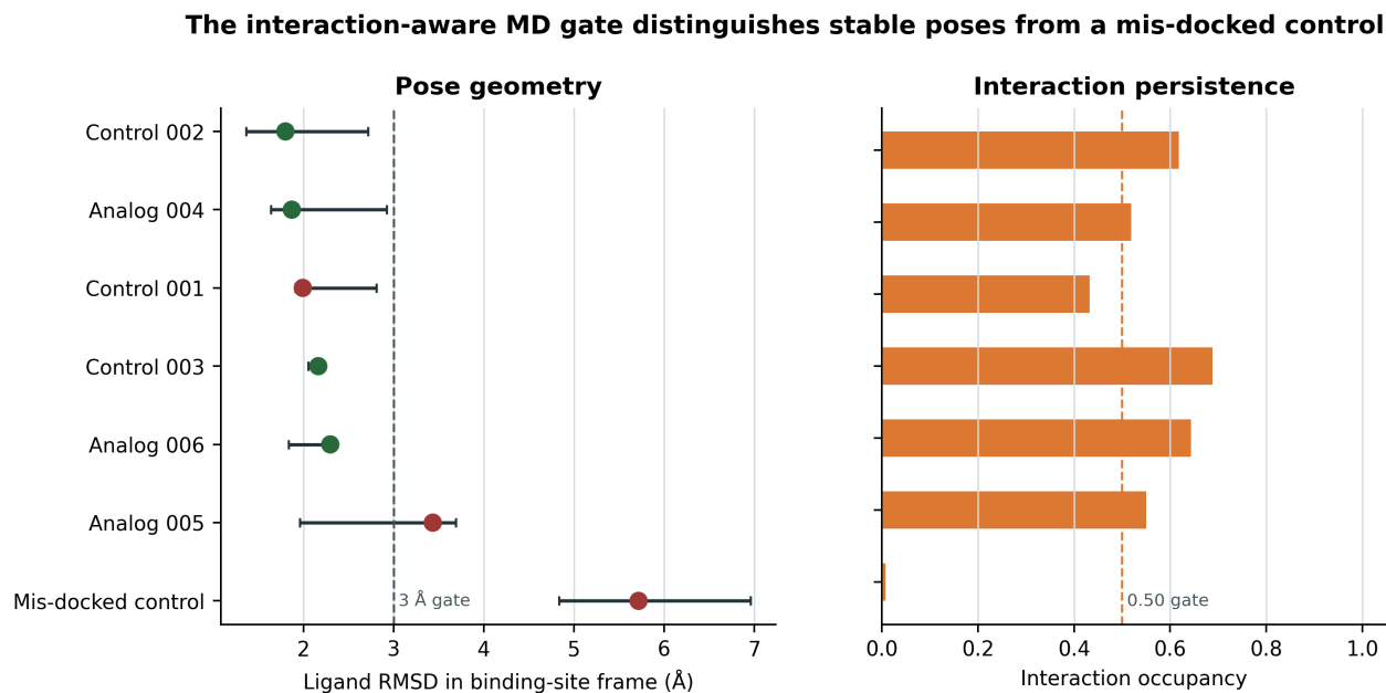
Figure 6: MD pose-persistence stress test. Points summarize system-level median ligand RMSD and key-contact occupancy across three independent 20 ns production trajectories. Horizontal RMSD error bars show the across-replicate range of replicate-level median ligand RMSD; colors indicate the predeclared majority-replicate decision.
