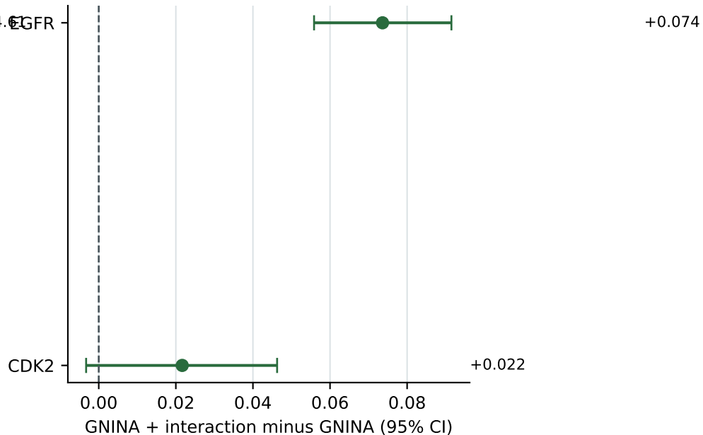
BEDROC difference
