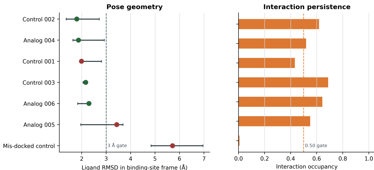
Figure 6: MD pose-persistence stress test. Points summarize system-level median ligand RMSD and key-contact occupancy across three independent 20 ns production trajectories. Horizontal RMSD error bars show the across-replicate range of replicate-level median ligand RMSD; colors indicate the predeclared majority-replicate decision.
