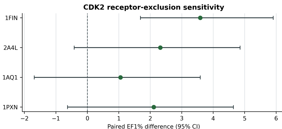
Figure 5: CDK2 receptor-exclusion sensitivity. Points show paired EF1% differences and horizontal bars show paired 95% confidence intervals after exclusion of one receptor from the four-receptor CDK2 transfer ensemble.
