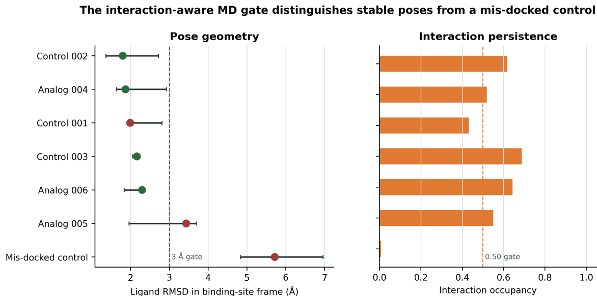
Figure 6: MD pose-persistence stress test. Points summarise candidate-level median ligand RMSD with the range across three independent 20 ns replicates; bars show candidate-level median core-contact occupancy. Colours indicate the predeclared majority-replicate decision. The deliberately mis-docked control is separated from the majority-stable systems by both geometric and interaction evidence. Full-protein start/end coordinate renders for the stable and failed examples are retained in the public repository.
