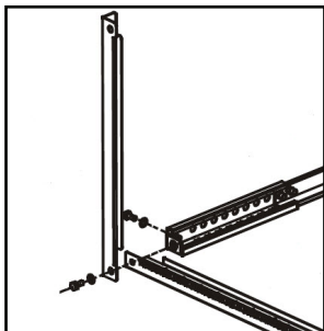
Aligning the Top Bracket with the Vertical Rail
