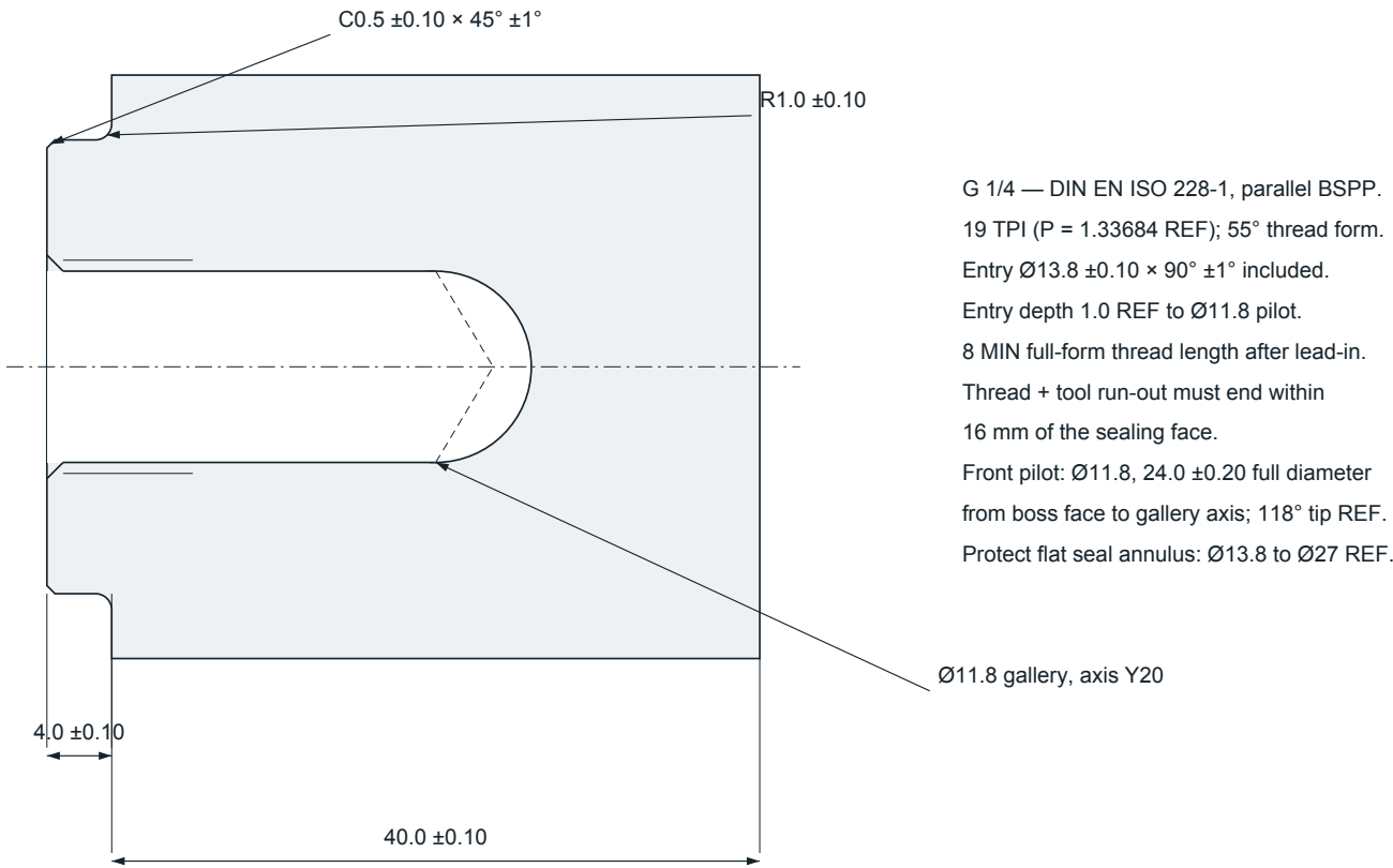
DETAIL A — FRONT G 1/4 PORT / BOSS, 2:1 (20 places)
