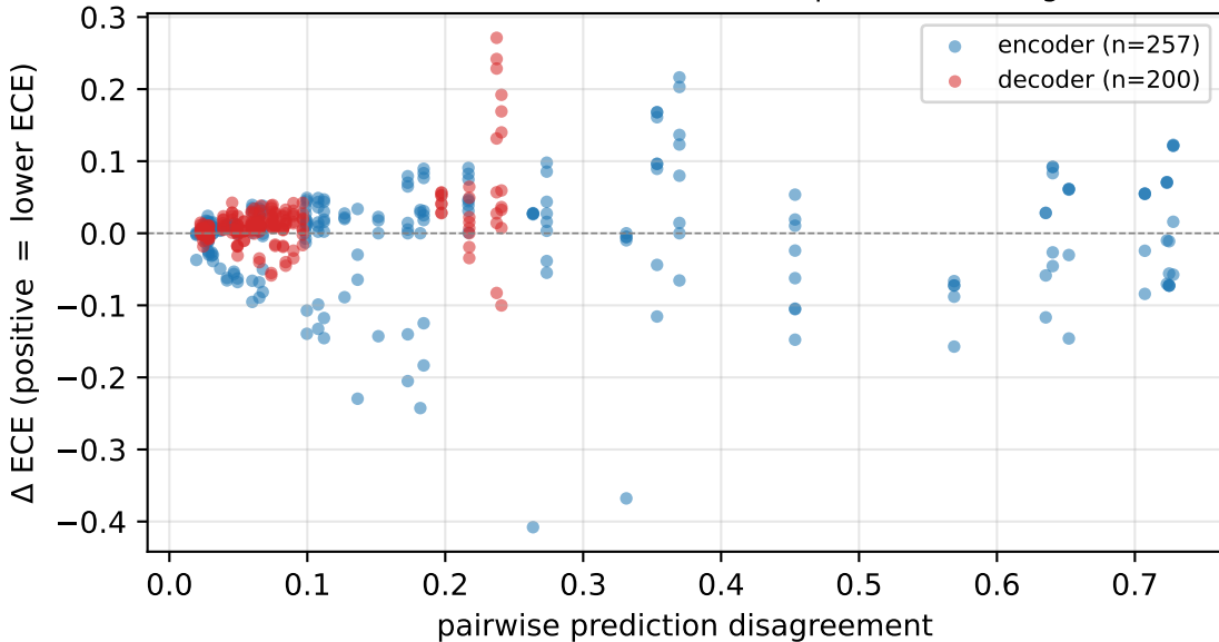
Frontier (calibration arm): both families improve with disagreement
