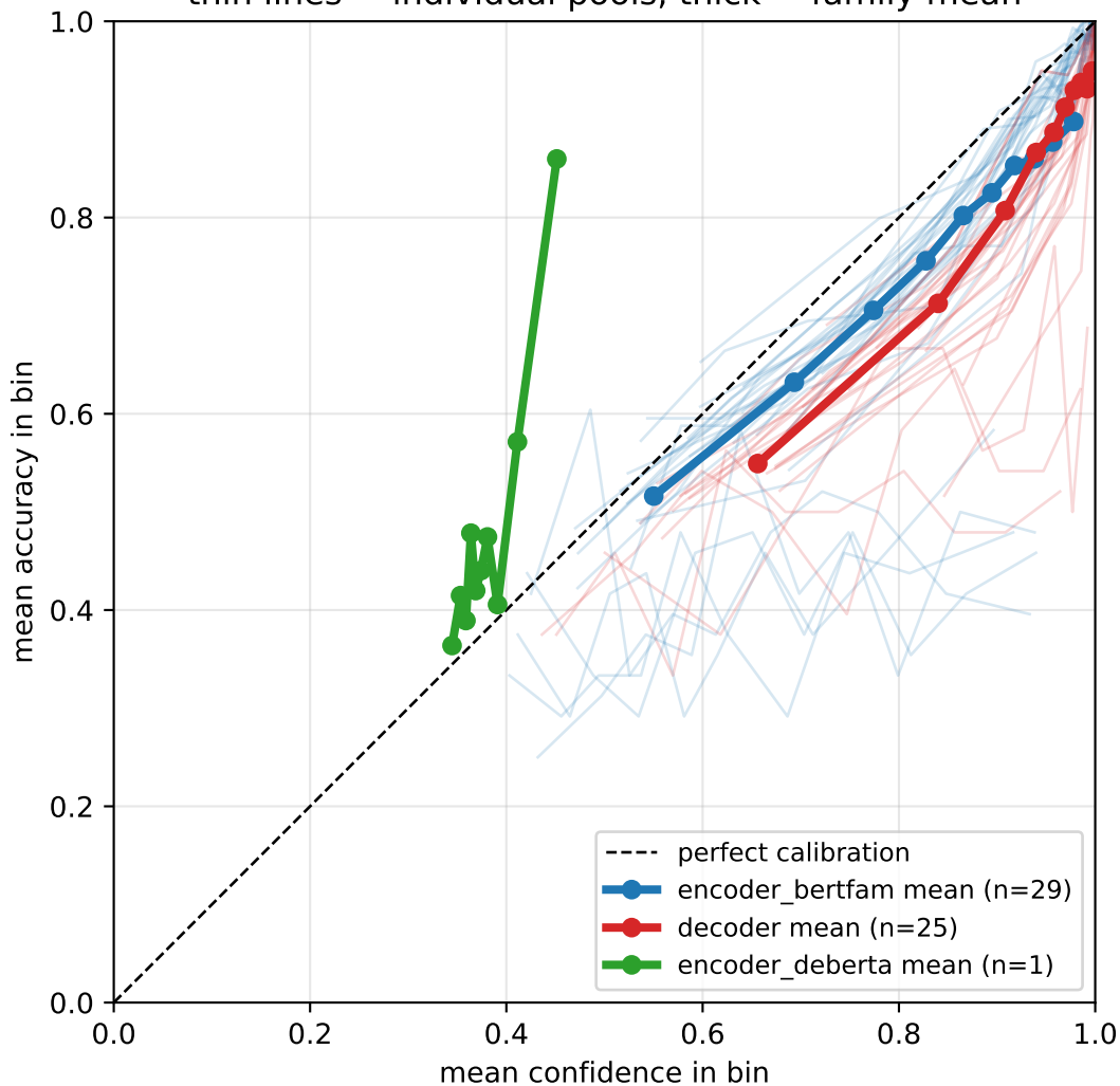
Per-pool reliability diagrams (best_single) thin lines = individual pools, thick = family mean
