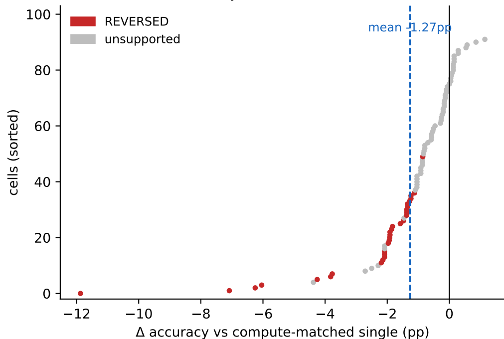
B Strict encoder comparison: 0/92 SUPPORTED, 31 REVERSED
