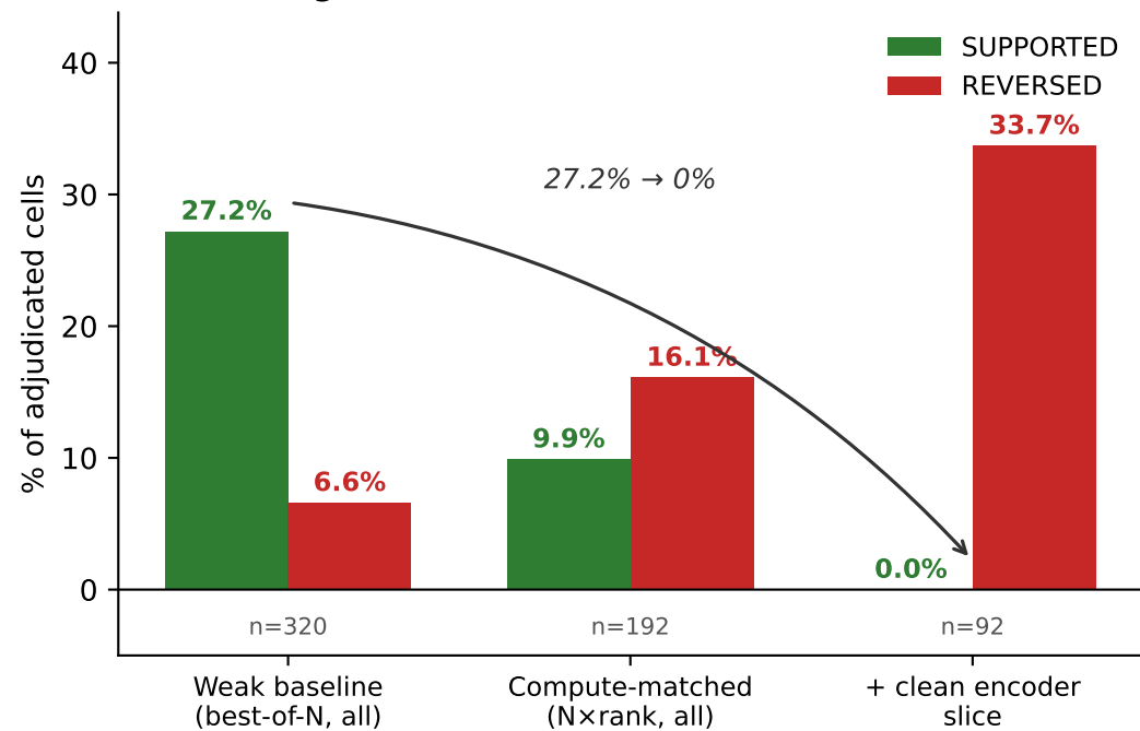
A Removing evaluation shortcuts erases the benefit
