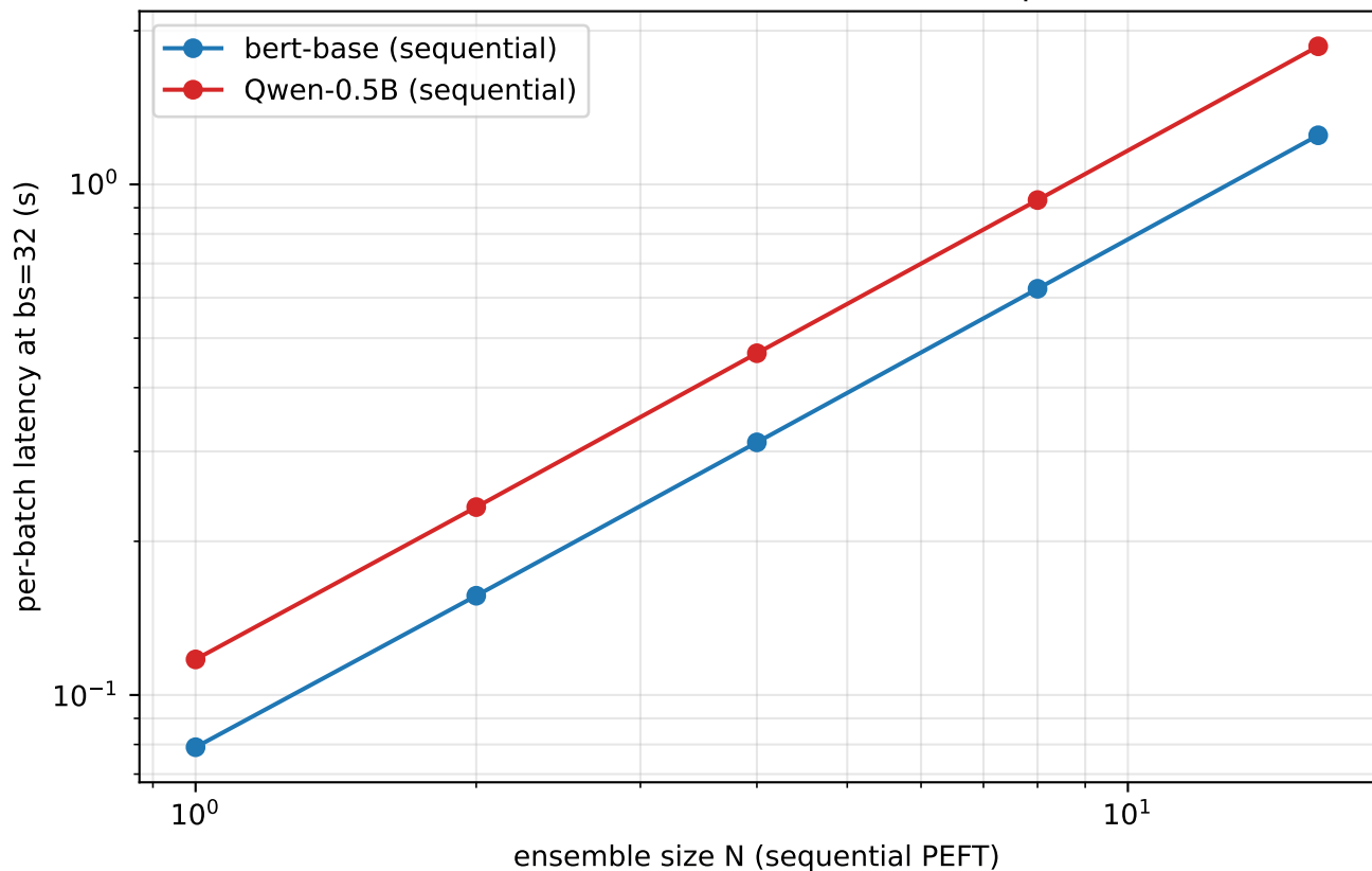
Linear cost of sequential ensemble inference (vLLM multi-LoRA would amortize, ~2-3x predicted)
