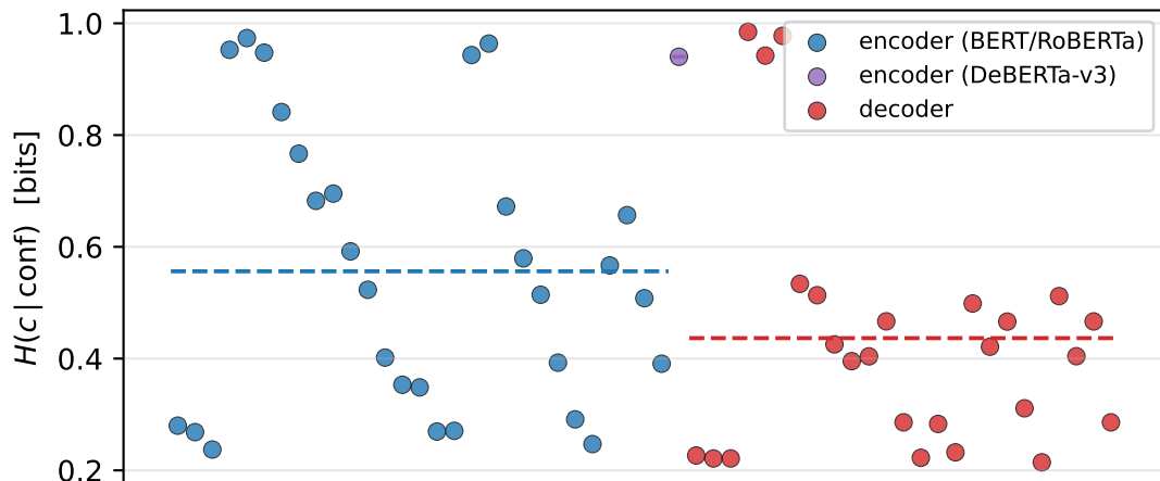
Per-pool mutual information between correctness and confidence
