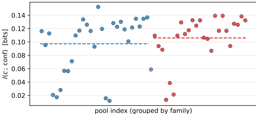
Per-pool mutual information between correctness and confidence
