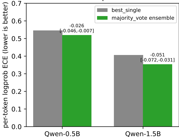
Calibration: ECE drop doubles with scale
