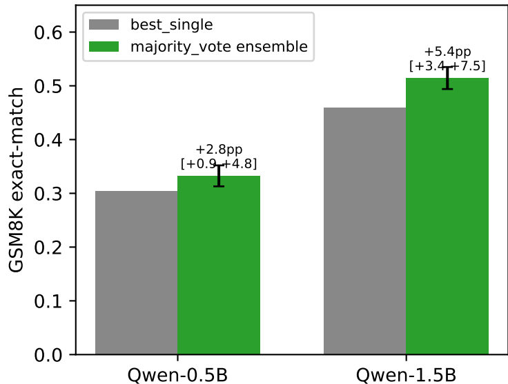
Accuracy: ensemble effect doubles with scale
