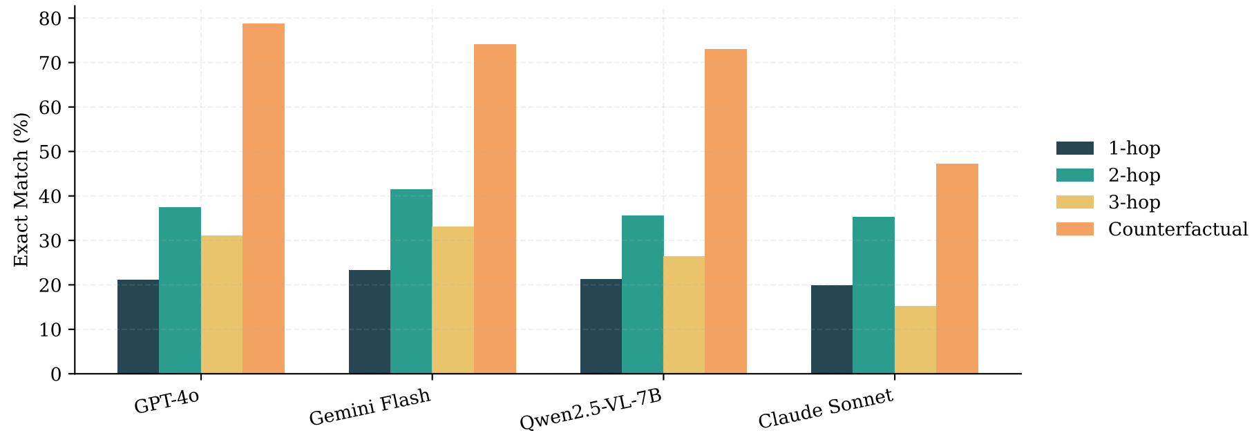
Difficulty-Level Breakdown
