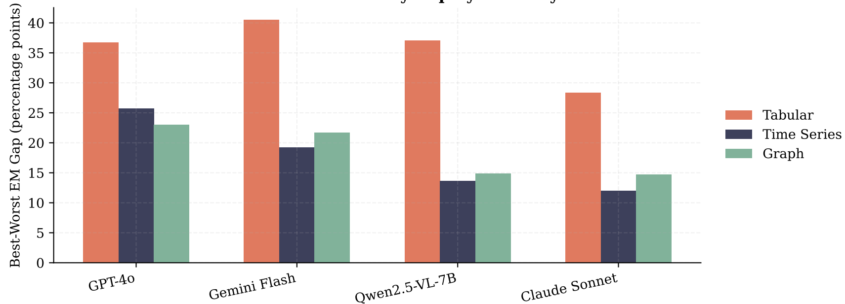
Visualization Sensitivity Gap by Modality
