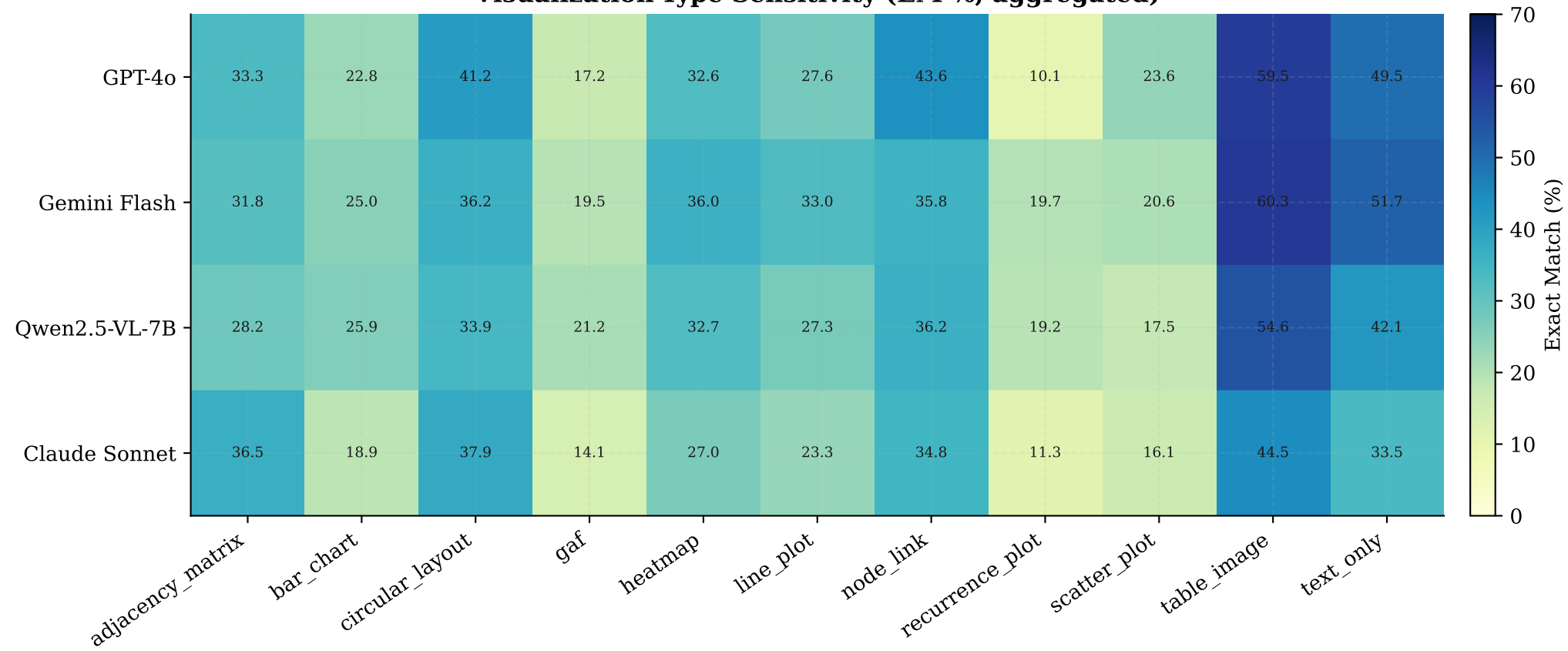
Visualization-Type Sensitivity (EM %, aggregated)
