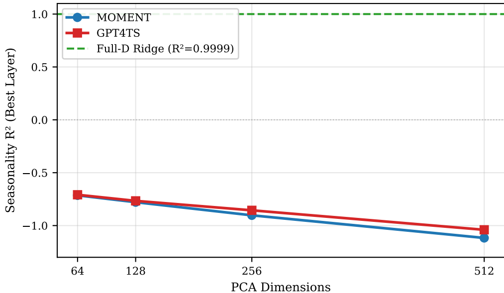
PCA Dimension vs. Seasonality R^2
