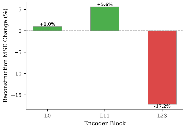
Erasing Trend
