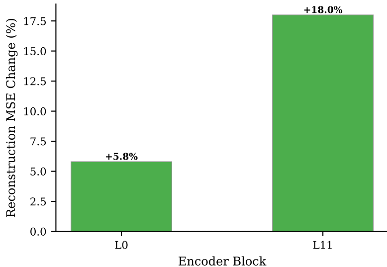
Erasing Stationarity
