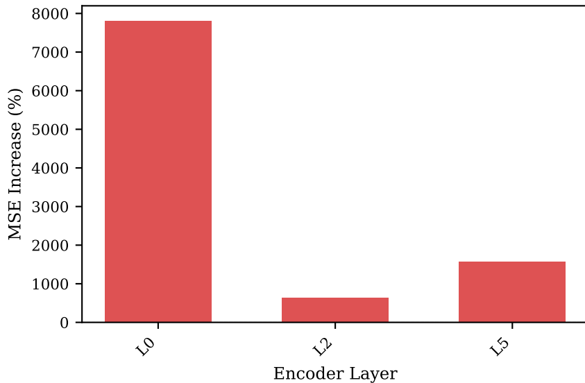
Erasing Trend
