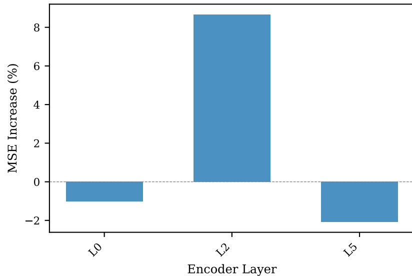
Erasing Stationarity
