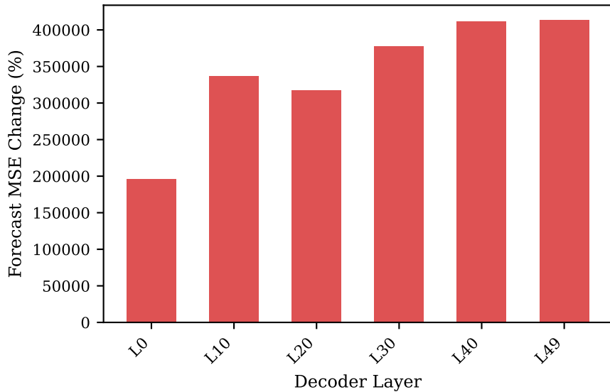
Erasing Trend
