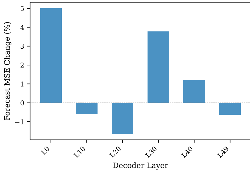
Erasing Stationarity
