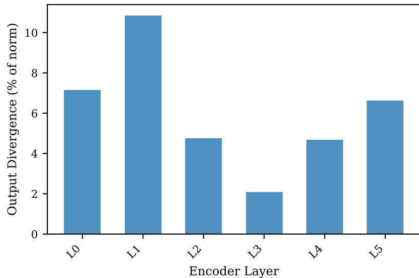
Erasing Stationarity
