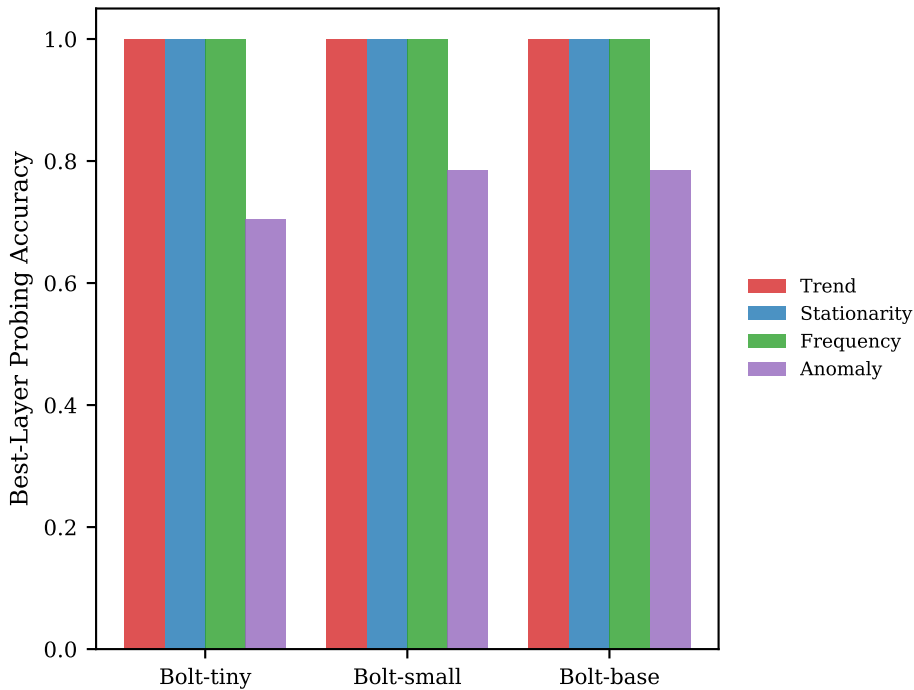
Scaling Analysis: Chronos-Bolt (Tiny \rightarrow Small \rightarrow Base)
