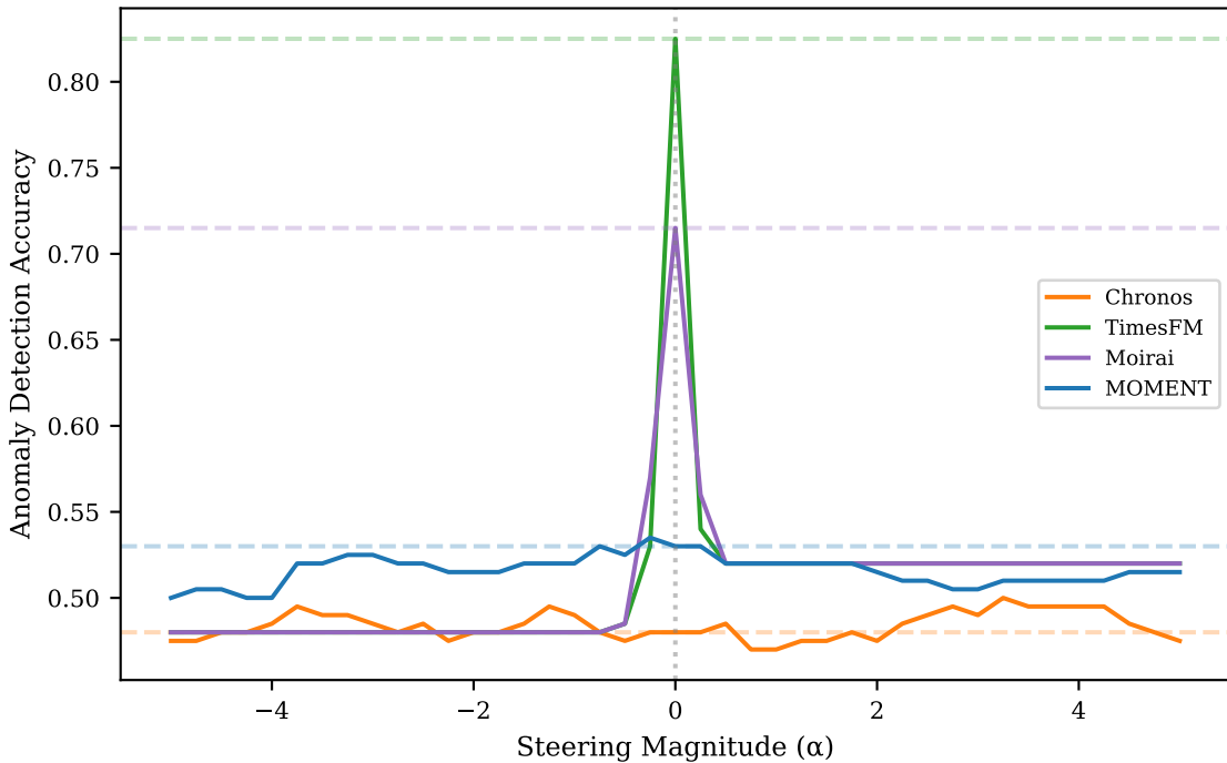
LDA Steering for Anomaly Improvement
