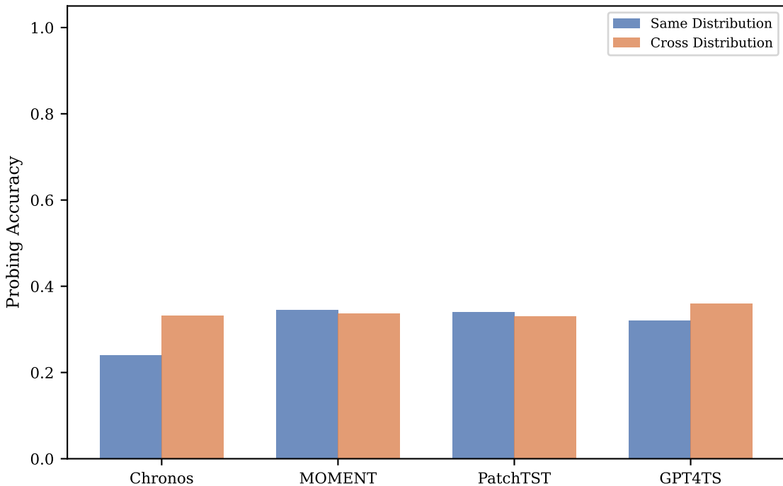
Cross-Dataset Transfer: Trend Probing
