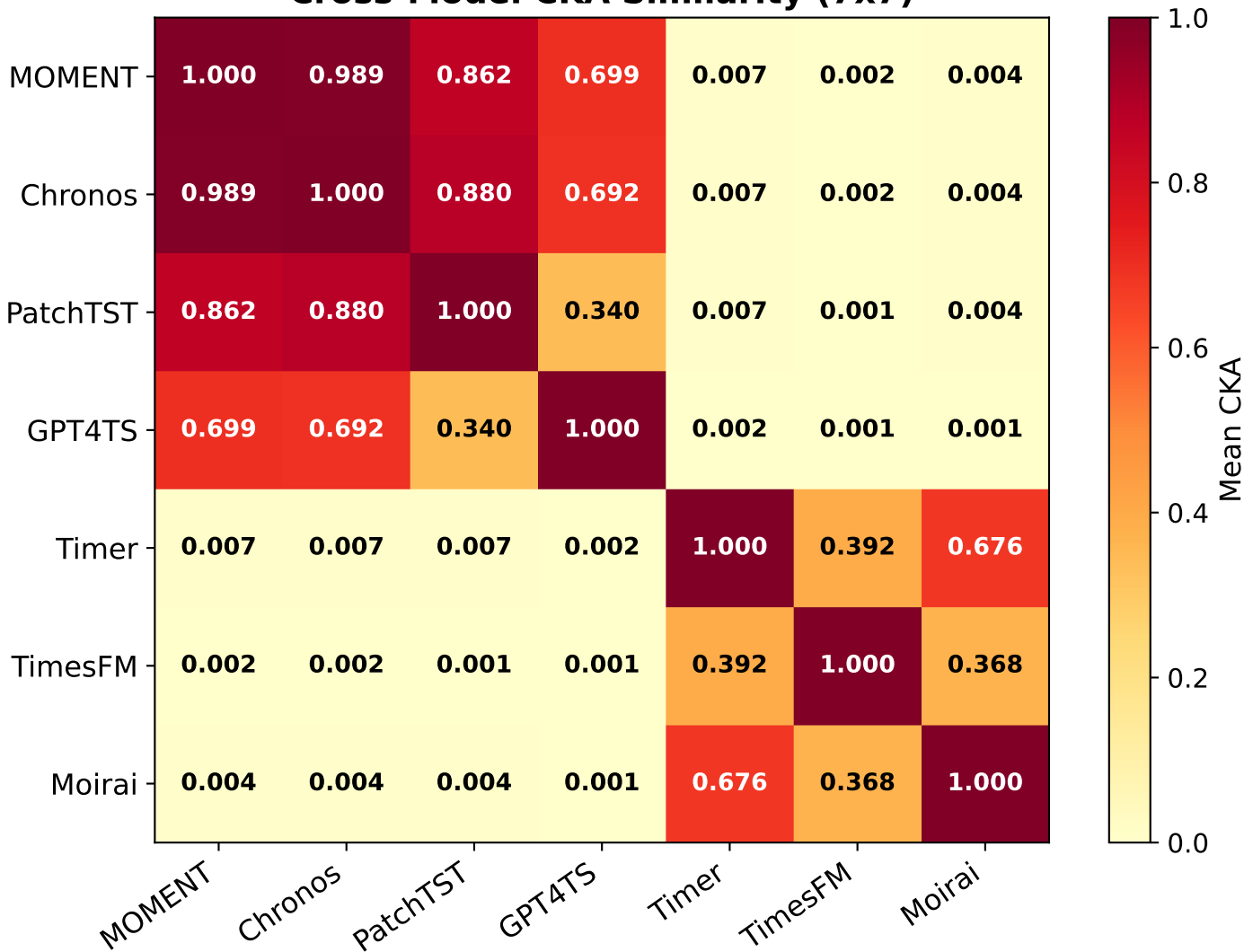
Cross-Model CKA Similarity (7x7)
