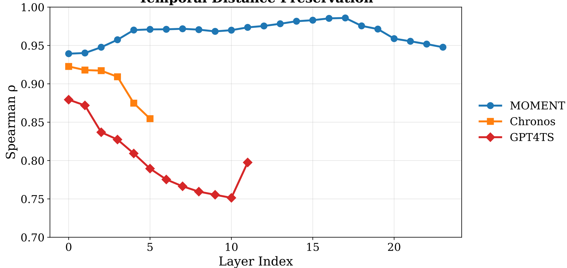
Temporal Distance Preservation
