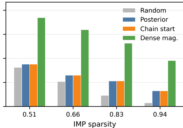
Fashion-MNIST
