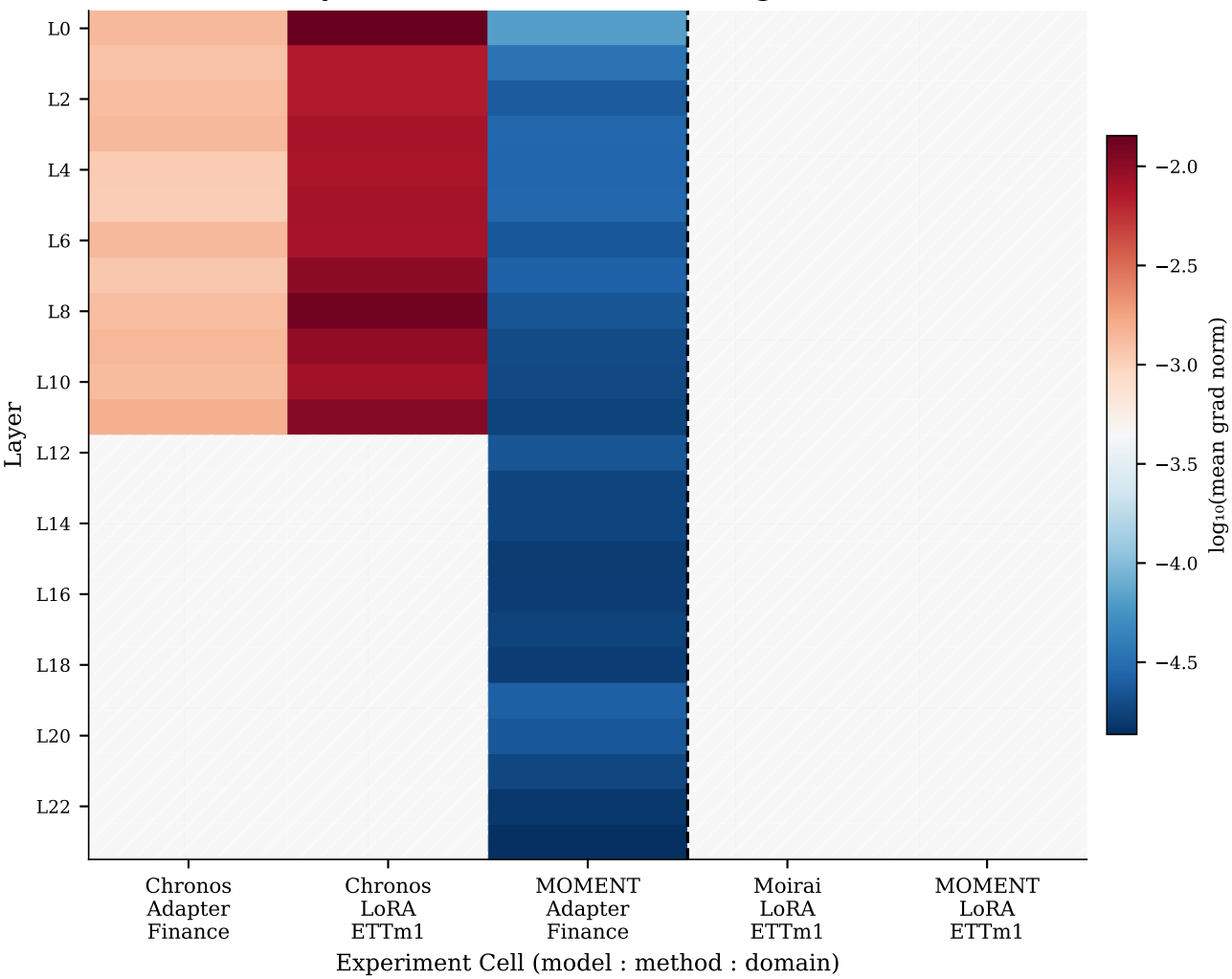
Layer-wise Gradient L2 Norm ( \log_{10} scale)
