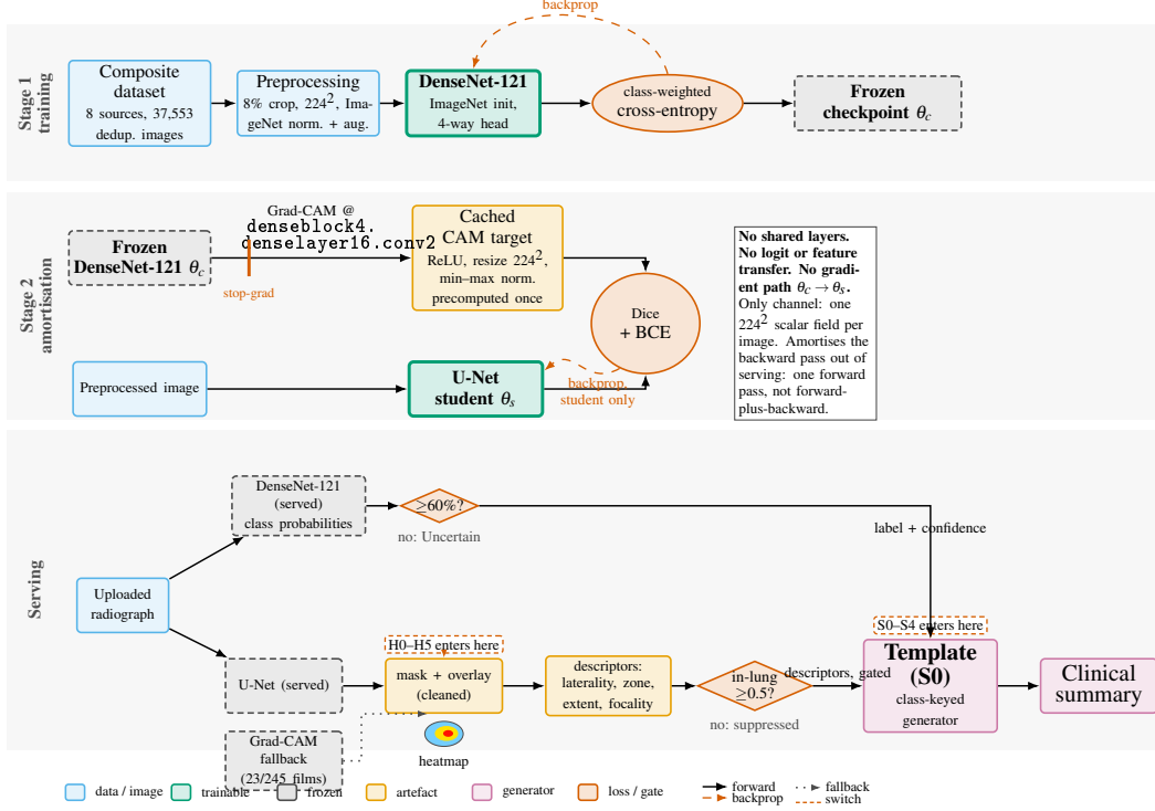
Figure 1: System overview. Stage 1 trains the served DenseNet-121 classifier. Stage 2 supervises a U-Net student on Grad-CAM targets cached from the frozen classifier (stop-gradient marked): no layers, logits, or features are shared, so the only channel is one 224 \times 224 scalar field per image, amortising the backward pass out of serving. At inference the classifier supplies label and confidence; the localiser supplies gated region descriptors; both arrive at the report generator, a class-keyed template (S0), which alone determines the printed summary. Tags mark where H0–H5 and S0–S4 enter.
