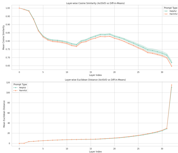
Figure 8: Cosine similarity and Euclidean distance between ActSVD and DIM jailbroken model activations. This comparison examines how the two editing methods differ from each other across all 33 layers
