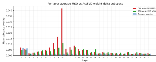
Figure 2: Average per-layer MSO between the DIM refusal direction and ActSVD weight-delta subspaces. Most layers are near the random baseline.
