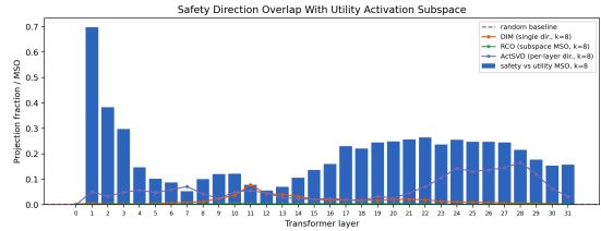
Figure 2: Per-layer safety-utility MSO at rank 8. Bars: full DIM mean-difference direction at each layer ( 98 \times random on average). Lines: each method’s safety object projected onto the same utility PCA basis. RCO’s 2-D cone subspace MSO (green) tracks the random baseline at every layer.
