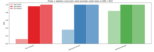
Figure 6: Ablation cross-test: same probe prompts under base vs each ablated model. Both DIM (1-D direction ablation) and RCO (2-D cone subspace ablation) are run as separate conditions on the same prompts. If RCO’s cone covers refusal directions DIM misses, RCO-ablated ASR should be at least as high as DIM-ablated ASR on every group.
