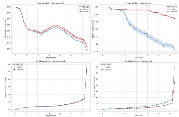
Figure 9: Cosine similarity and Euclidean distance between ActSVD and DIM jailbroken model activations and the Base model. Note the different Y axis scaling between the graphs
