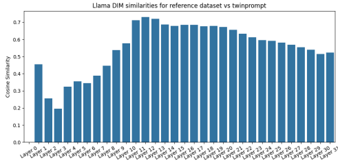
Figure 7: Difference-in-Means Self-Consistency
