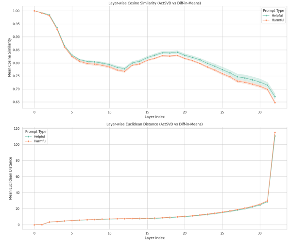
Figure 8: Cosine similarity and Euclidean distance between ActSVD and DIM jailbroken model activations. The first comparison examines how the two editing methods differ from each other across all 33 layers (embedding layer + 32 transformer blocks). In both cosine similarity and Euclidean distance, we observe that the two modified models produce clearly different internal representations. Harmful prompts are slightly more different than helpful, but not by a large margin. These findings are counter to what we would expect if these methods are truly only affecting safety, which would imply that each model would act similarly to the base model when prompted on helpful prompts.
