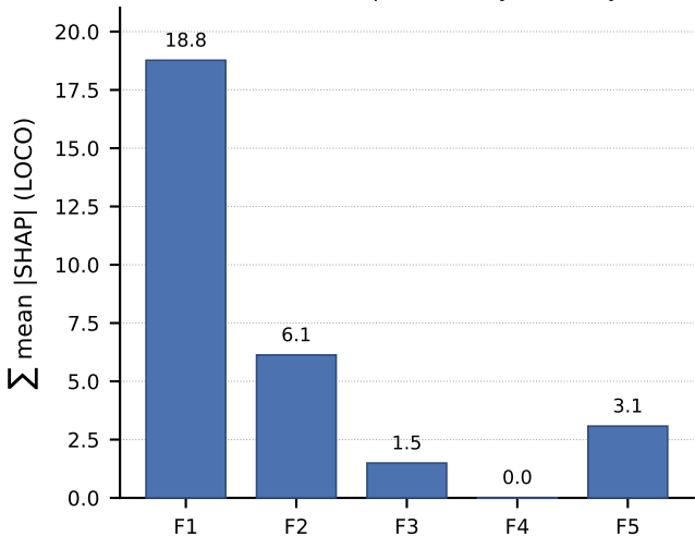
Global SHAP importance by modality
