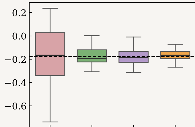
OLS
