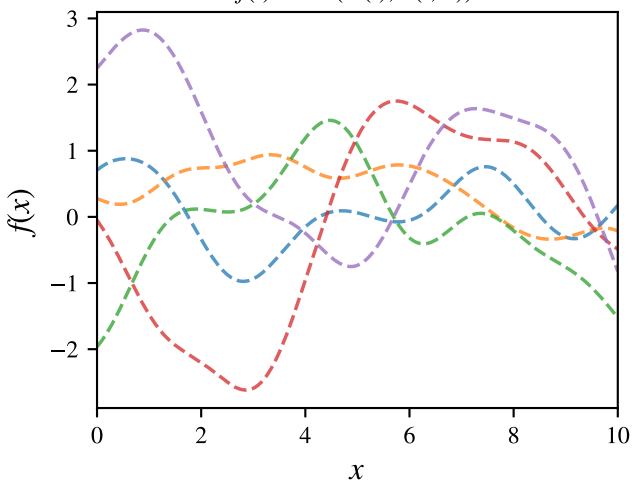
Gaussian Process Prior f(\cdot) \sim GP(m(\cdot), c(\cdot, \cdot))
