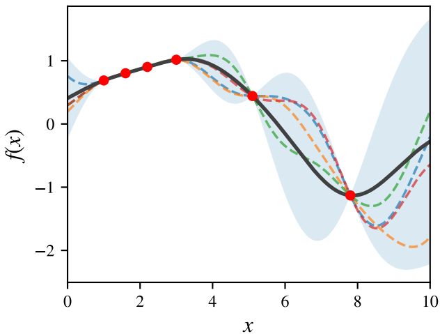
Posterior Prediction f(x) | \mathbf{f} \sim N(\hat{\mu}(x), \hat{\sigma}^2(x))
