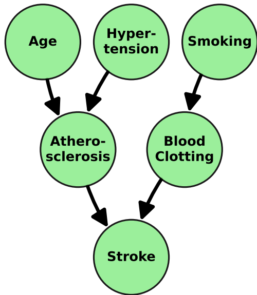
Ground Truth (5 edges)
