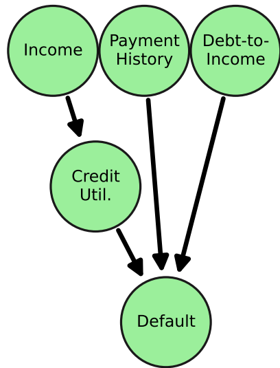
Ground Truth
